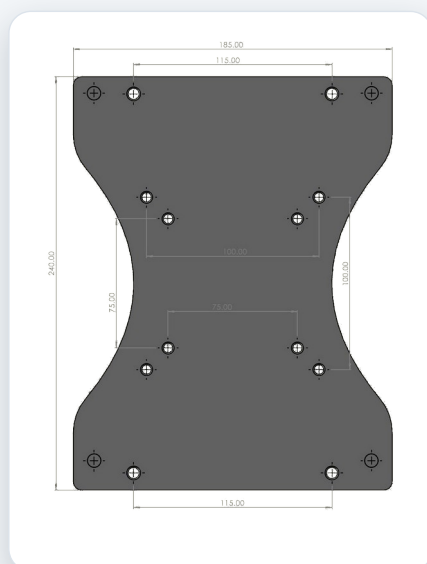
PLATE 185 × 240 MM
